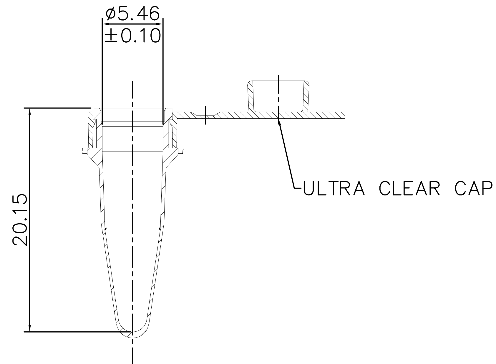
SECTION thro' TUBE & CAP 8pos
