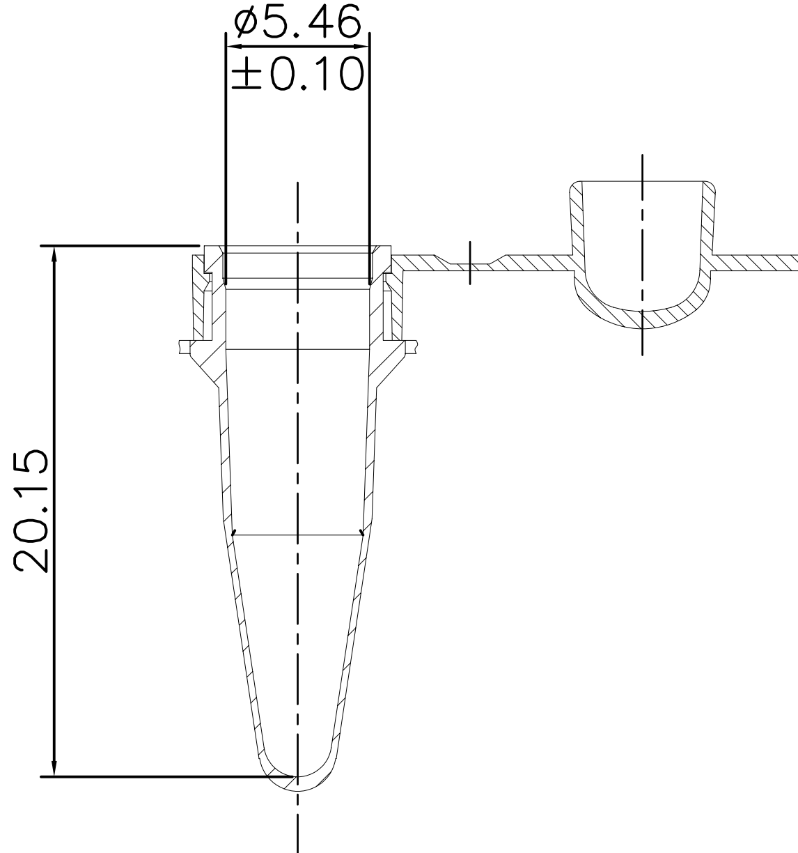
SECTION thro' TUBE & CAP 8pos
