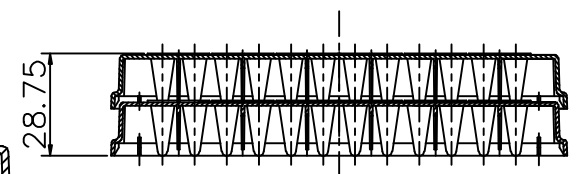
PLATES STACKED
