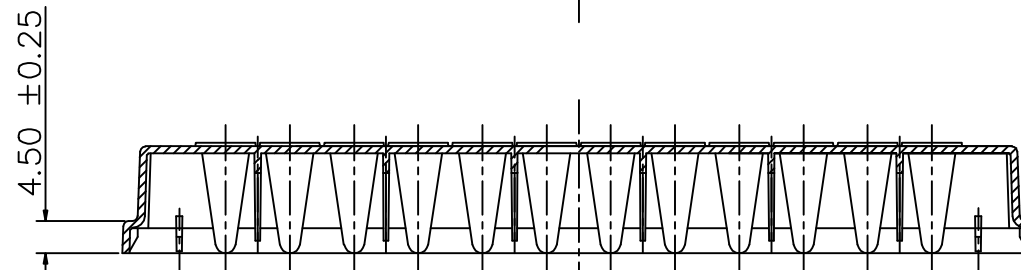
SECTION X-X
