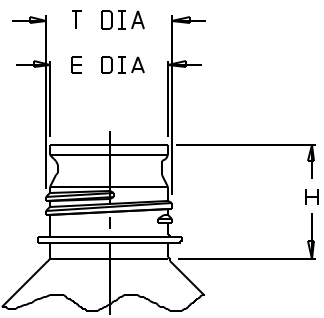
NECK DETAIL
